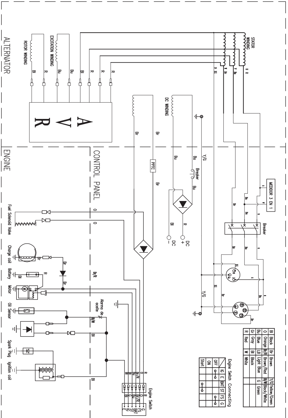
WIRING DIAGRAM OF 220V/230V/240V/380V/400V GENERATOR SET
